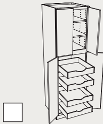
Utility with Roll Out Trays Block 5150
